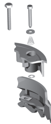
Bolt Down Detail
