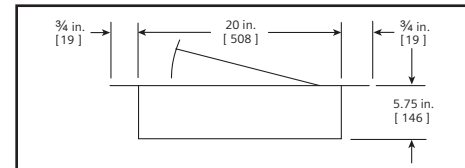
Flush Mounting
