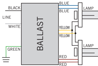
OMIT RED CONNECTION FOR SINGLE LAMP APPLICATION
