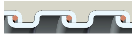
Square-Locked Design with integral bonding wire 3/8" through 1-1/4"
