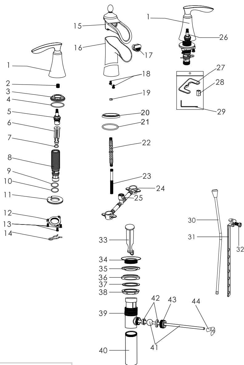
Cartridge (Type J)
