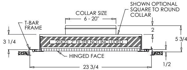
620TFG shown with optional square to round collar
