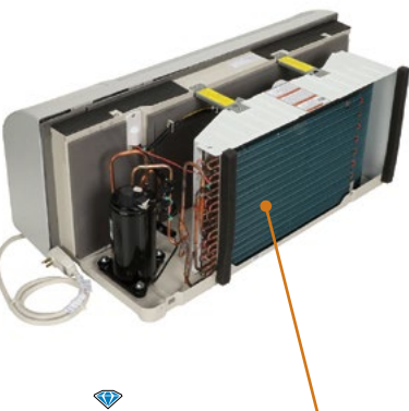
Outdoor curved coil is coated with Diamonblue Advanced Corrosion Protection®
