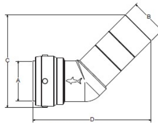
Street 45° Elbow
