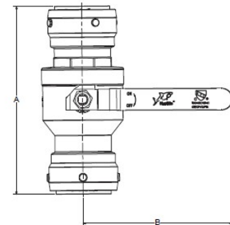
Ball Valve
