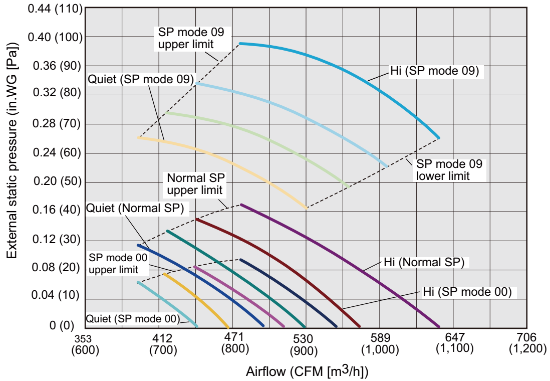
Available airflow rate range (High level)
