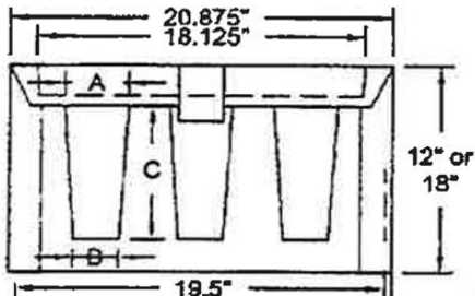
LENGTH VIEW
