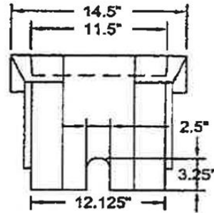
WIDTH VIEW
