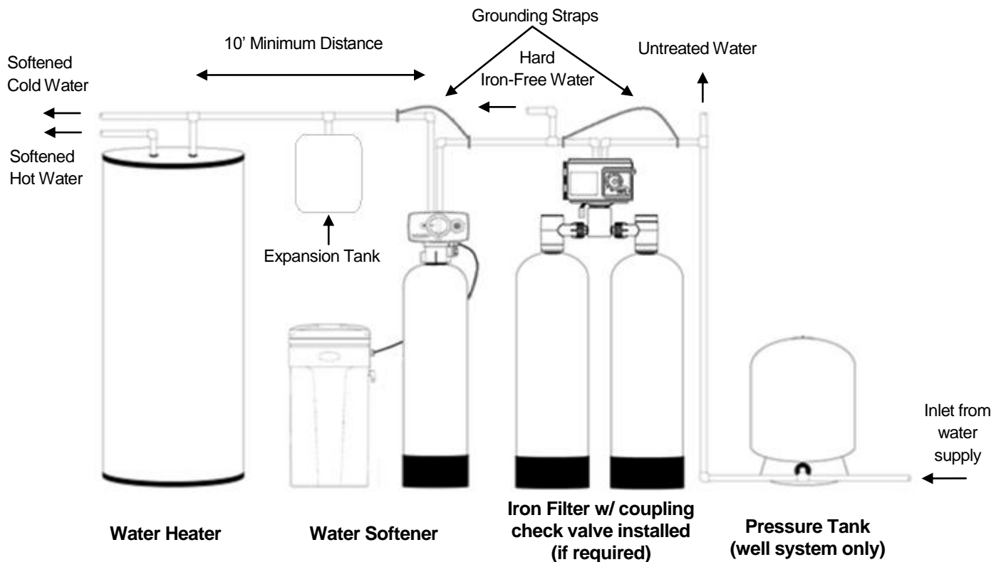
FIGURE 1: Typical Installation
