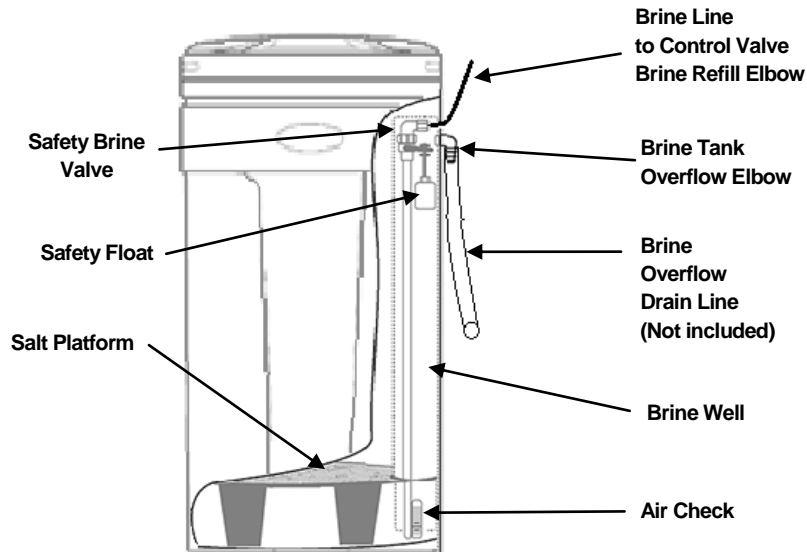
FIGURE 3: Brine Tank Components
