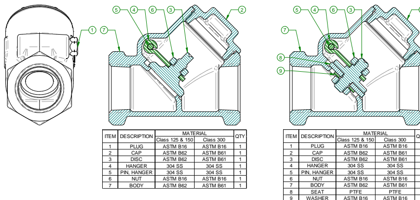
Type 3 Swing Check Valve
