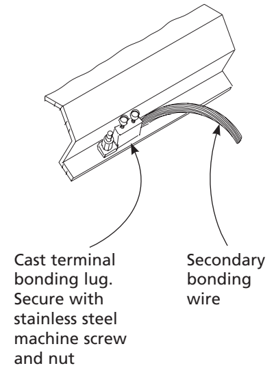
Typical Flashing Bond
