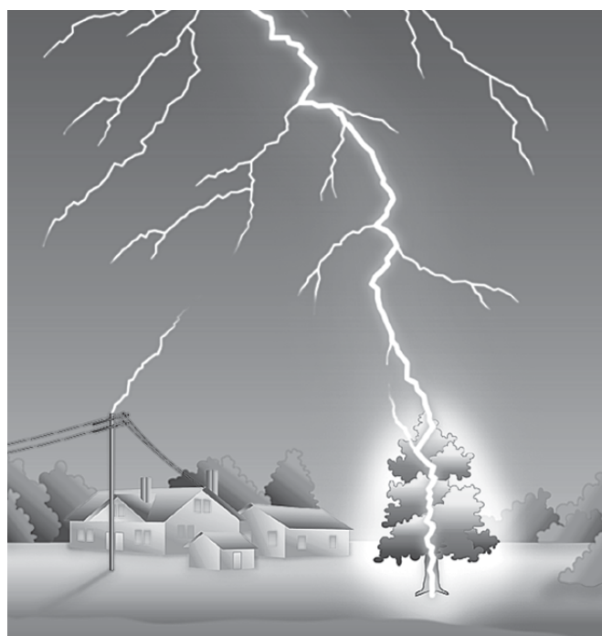
Figure 5. Upward leaders propagate toward downward leader to complete the ionized path between cloud and ground.
