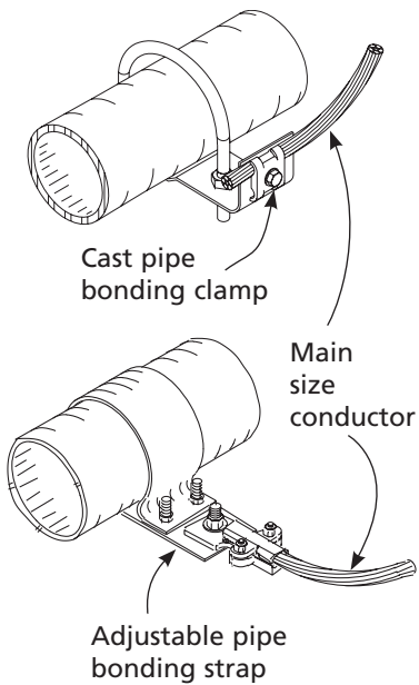
Typical Metallic Water Pipe Bonding Clamp
